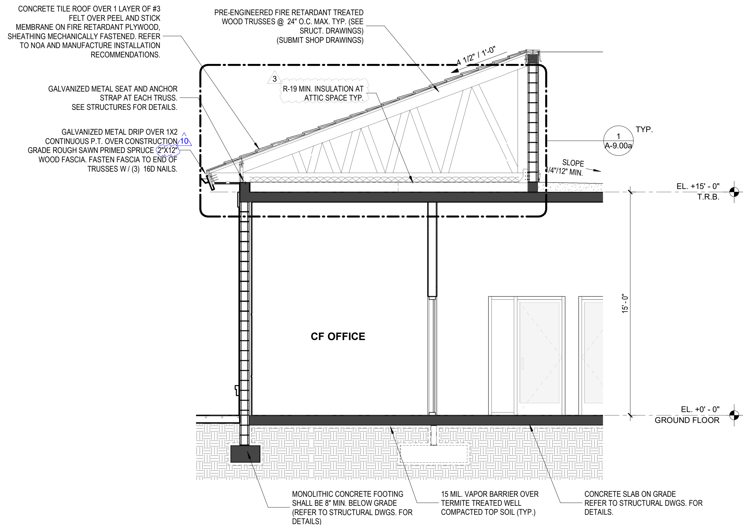
3 COMM. CENTER WALL SECTION 3 SCALE: 1/4" = 1'-0"
